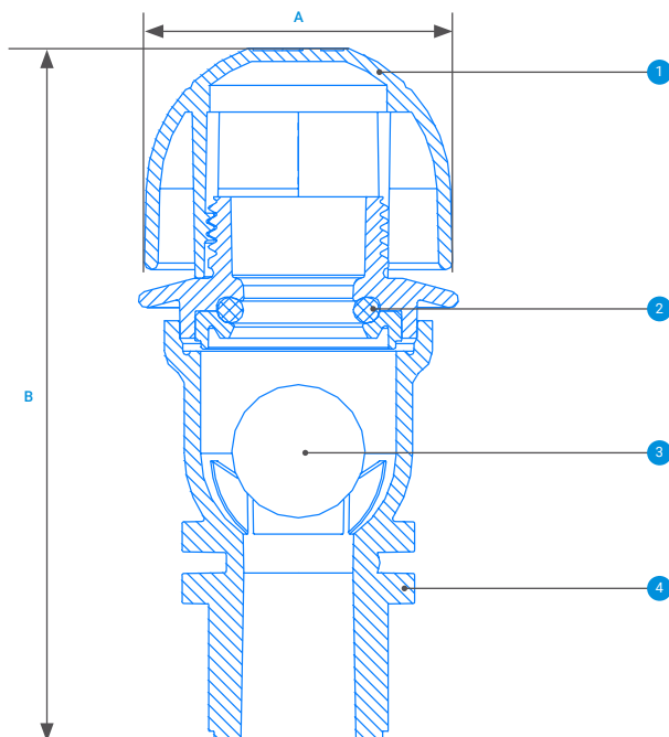
3/4", 1" Model
