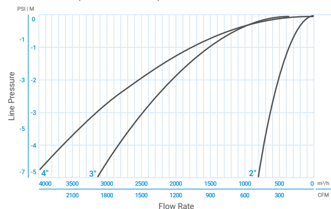
Inflow Data (Free Air Flow) 2", 3", 4"
