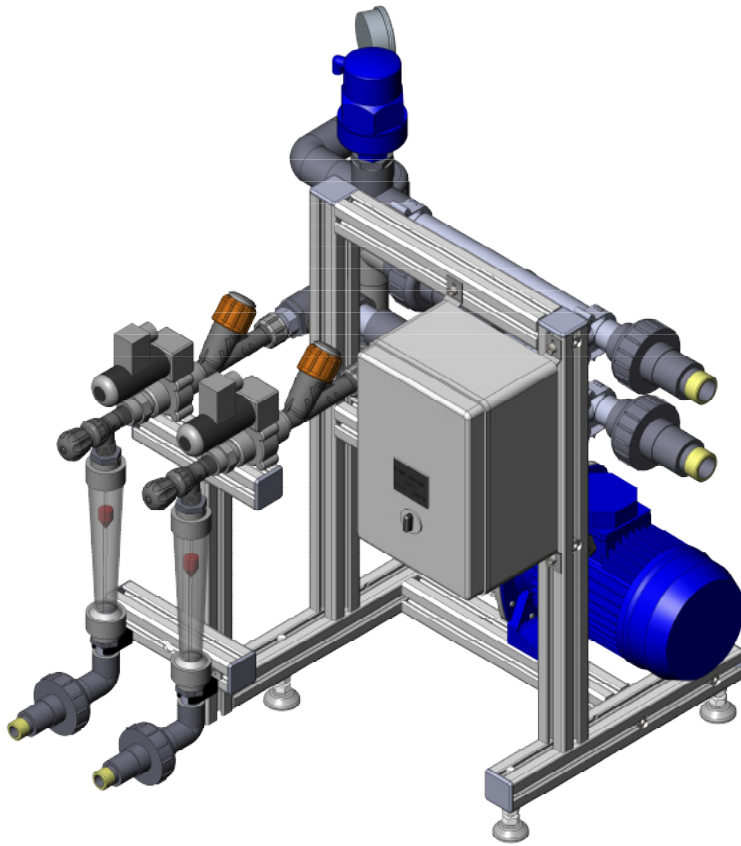
Typical setup
