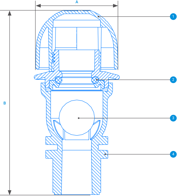
3/4", 1" Model
