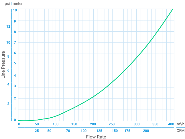
Discharge Data (Free Air Flow) - 2"
