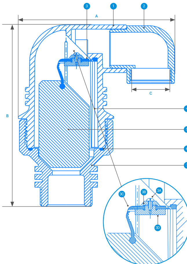
2" Model
