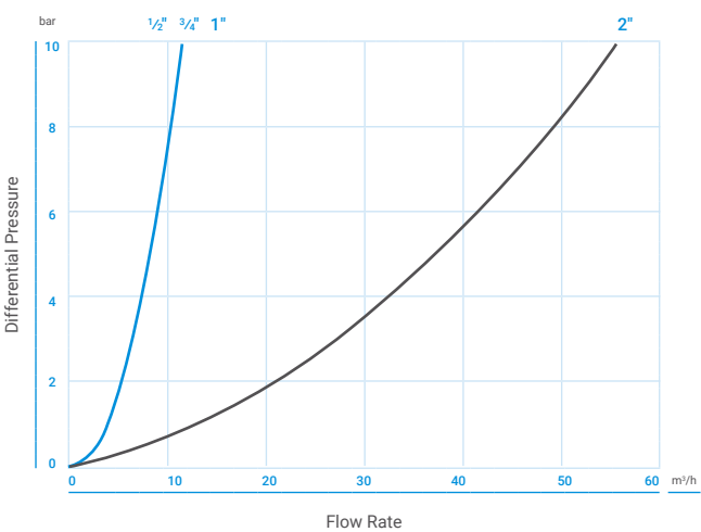
GD10 / PN 10 Automatic Air Release Flow Rate
