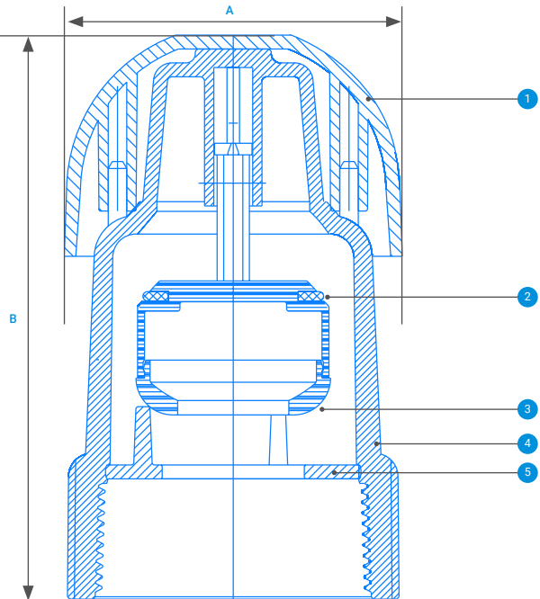
2" Model
