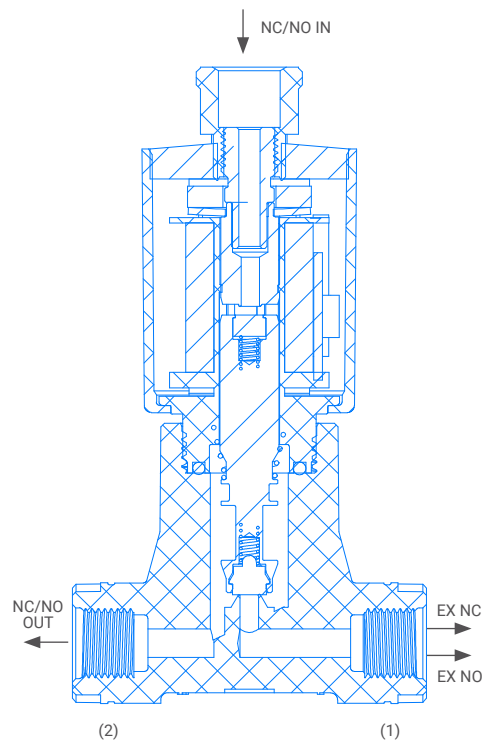
G75-A3P Model
