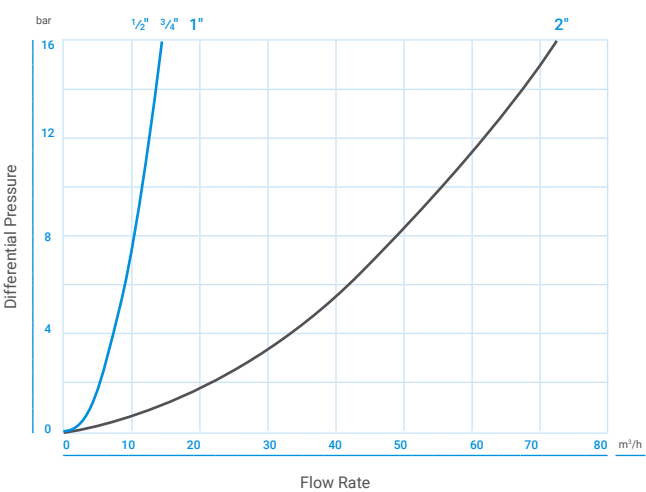
D40 / PN 16 Automatic Air Release Flow Rate
