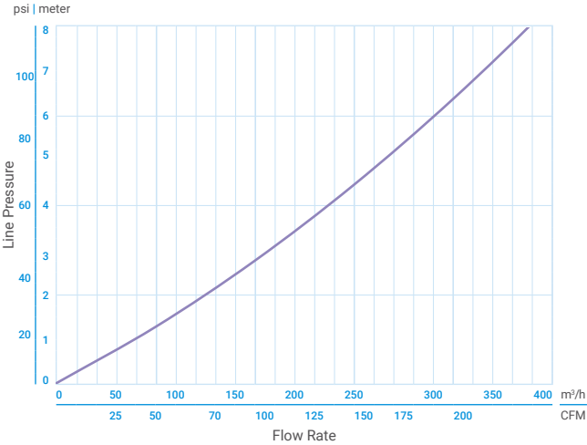
Discharge Data (Free Air Flow) Small Nozzle - 1/2", 3/4", 1", 2"
