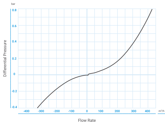
D43 NS Air & Vacuum Flow Rate
