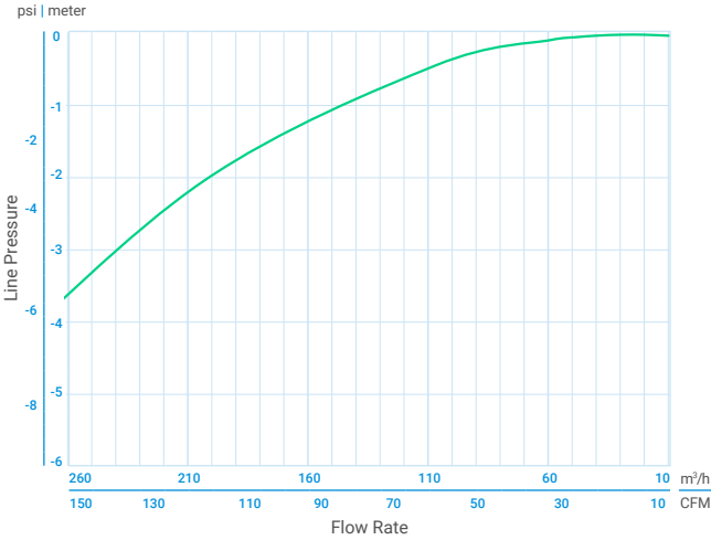
Inflow Data (Free Air Flow) - 2"
