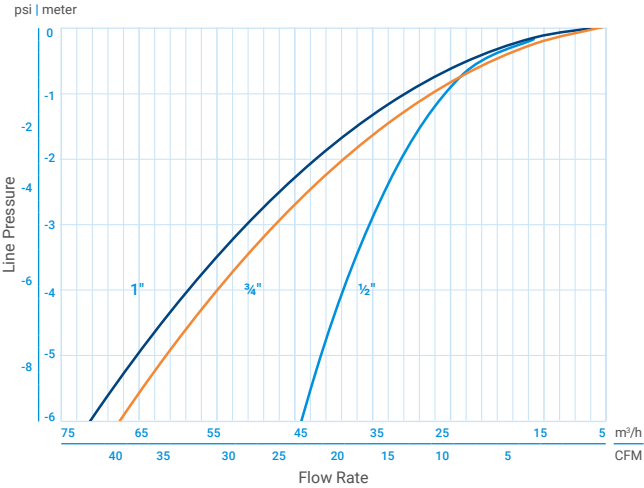
Inflow Data (Free Air Flow) - 1/2", 3/4", 1"
