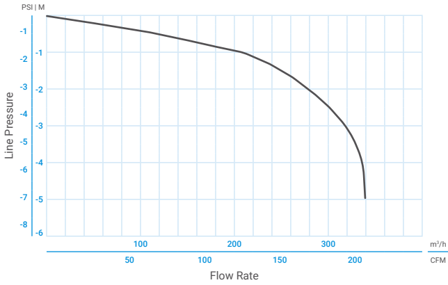
Inflow Data - Free Air Flow - 2"
